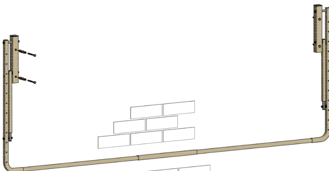
Figure 4 – Final Assembly
