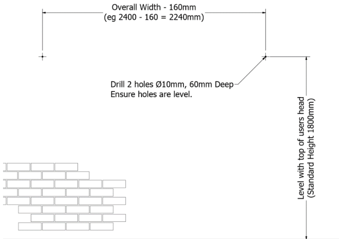
Figure 1 – Layout.
